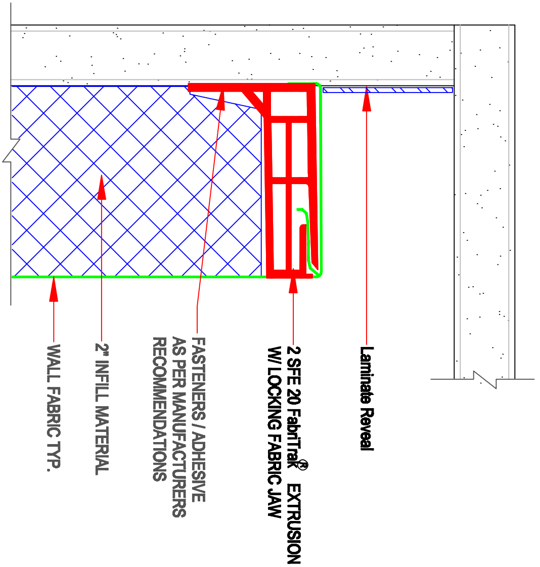
20.33 2 SFE 20 Laminate Reveal @ Inside Corner Scale: 1:1 Reference: Reveal
